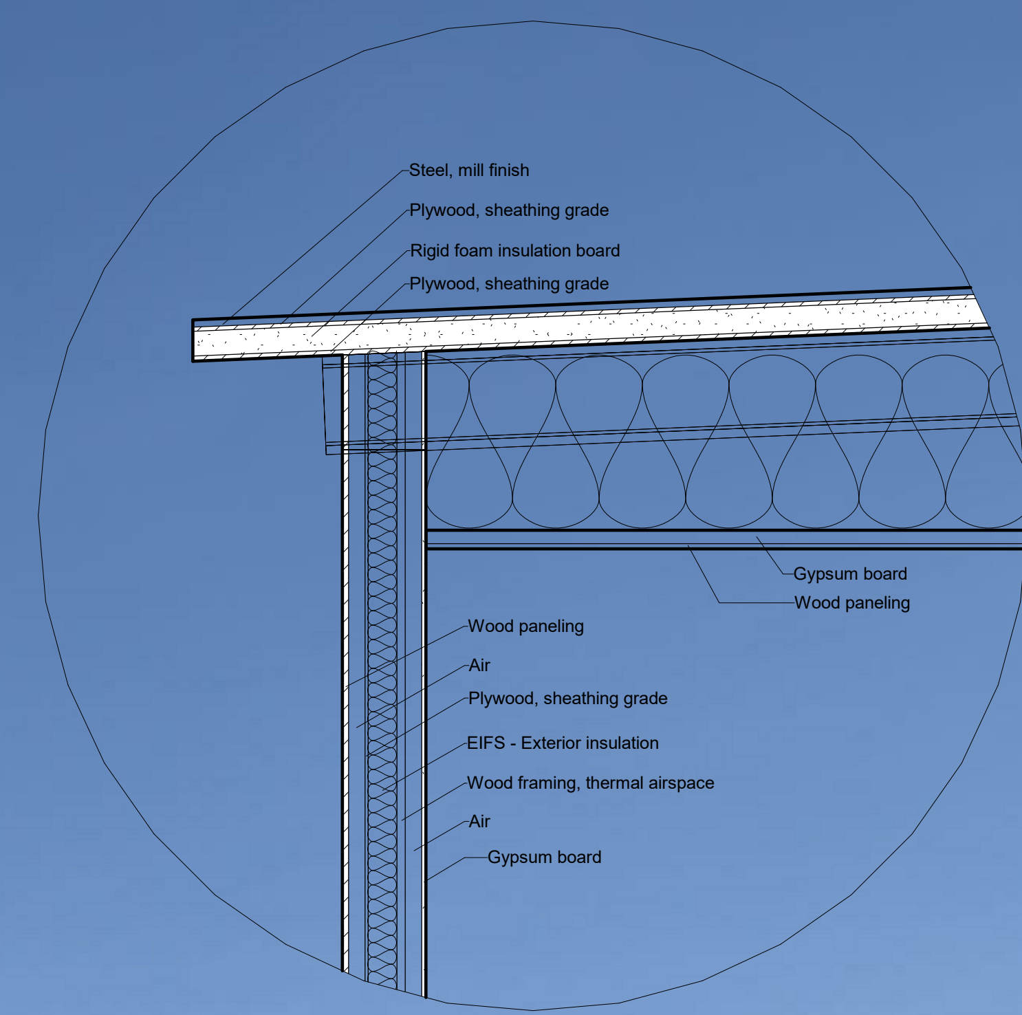
③ Roof + Wall Material Detail 3/4" = 1'-0"
