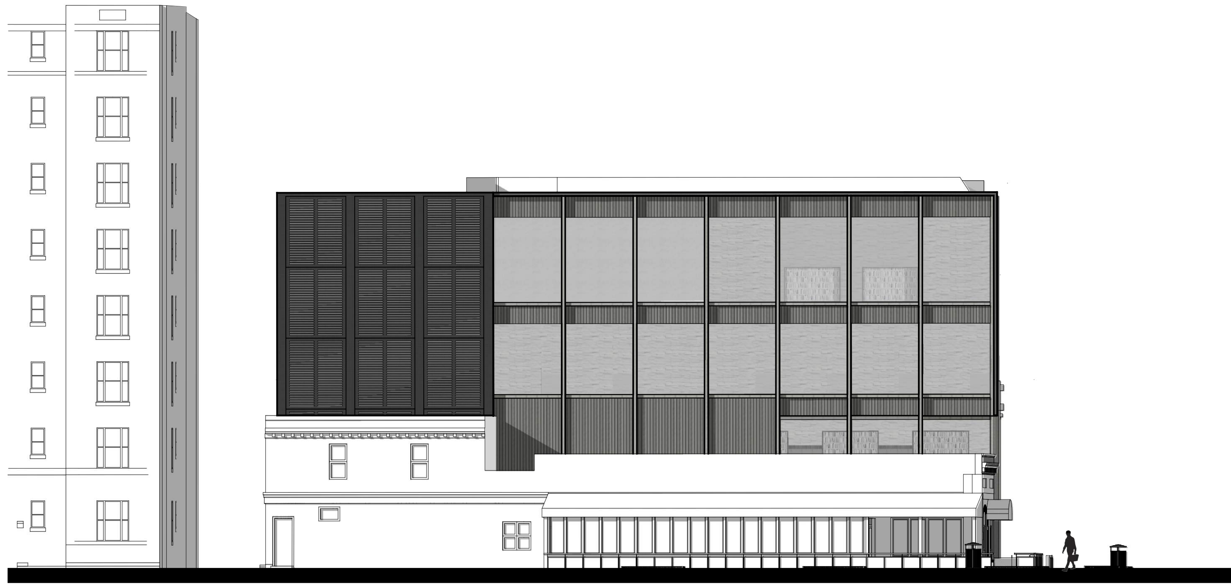
NORTH ELEVATION
