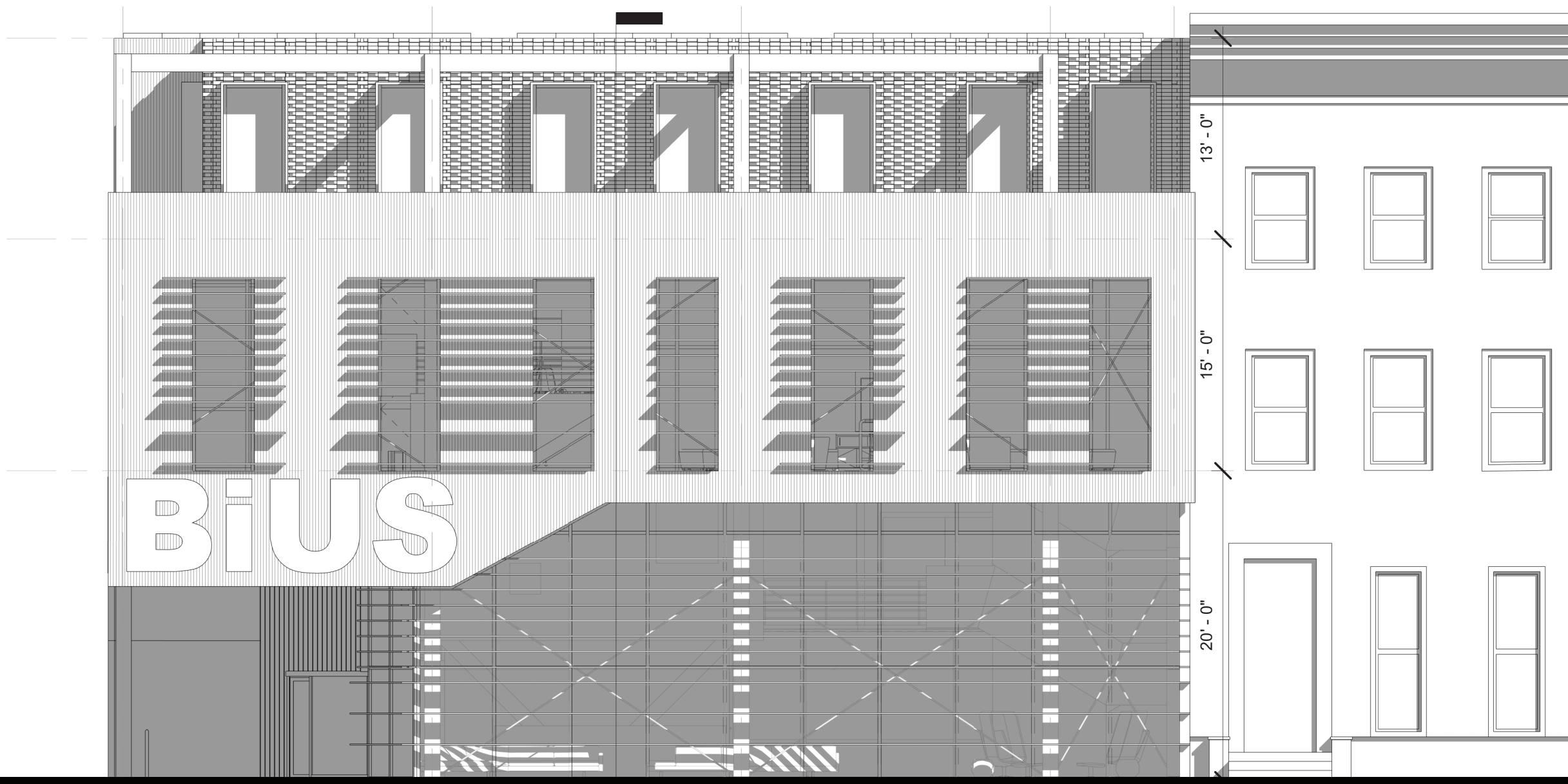
SOUTH ELEVATION : 1/8" = 1'-0"
