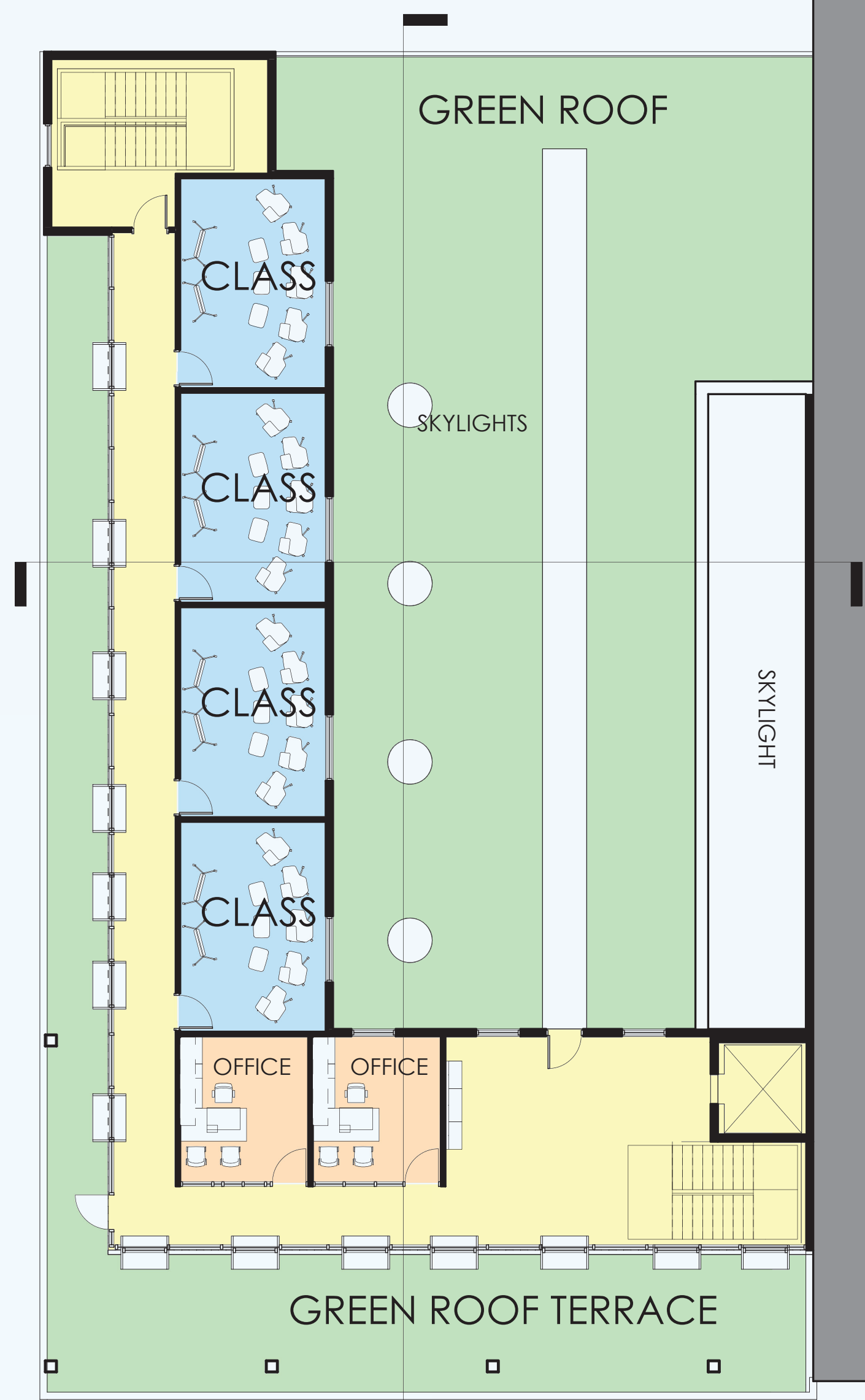
LEVEL 3 : 1/8" = 1'-0"
