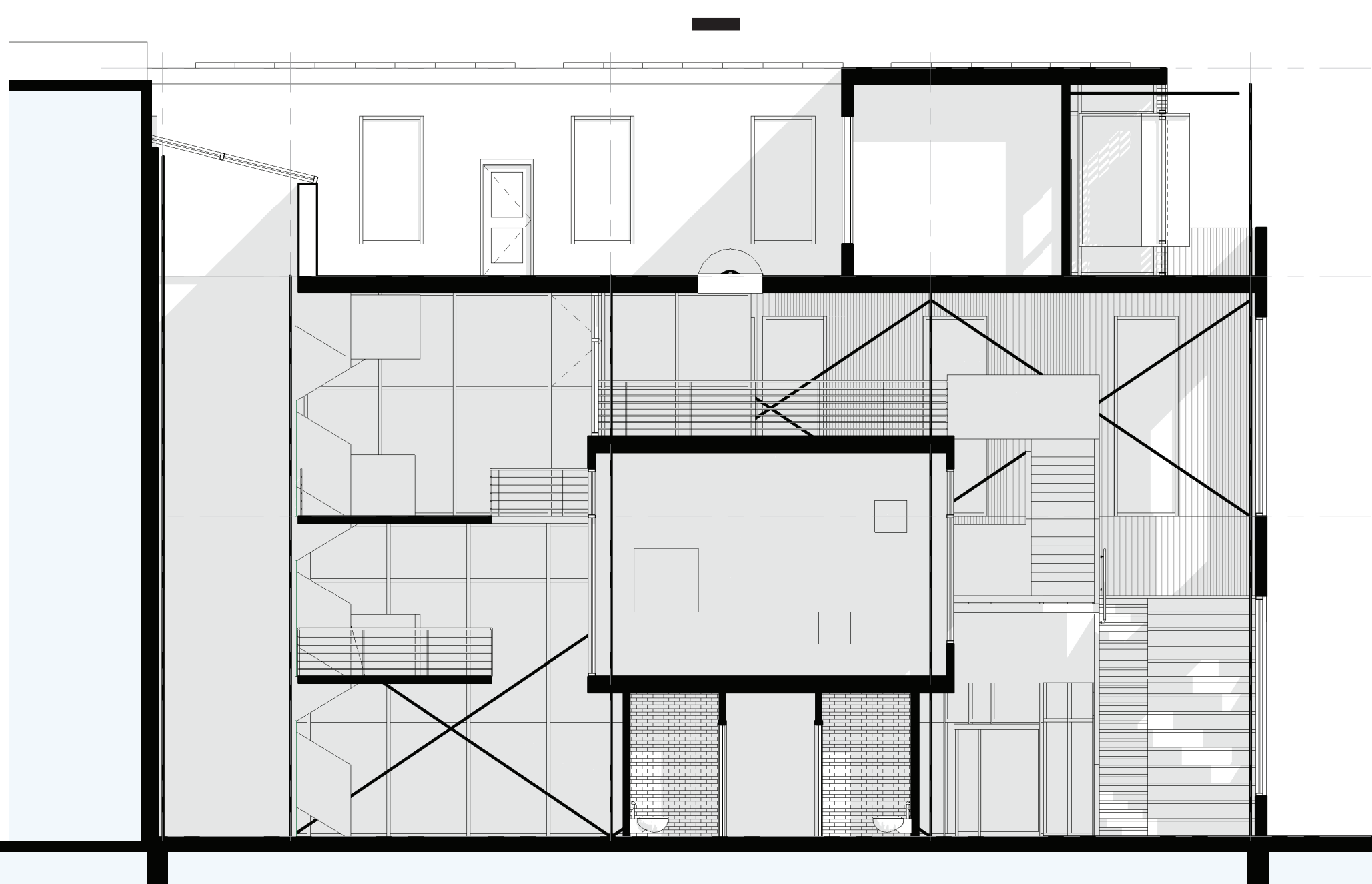
TRANSVERSE SECTION : 1/8" = 1'-0"
