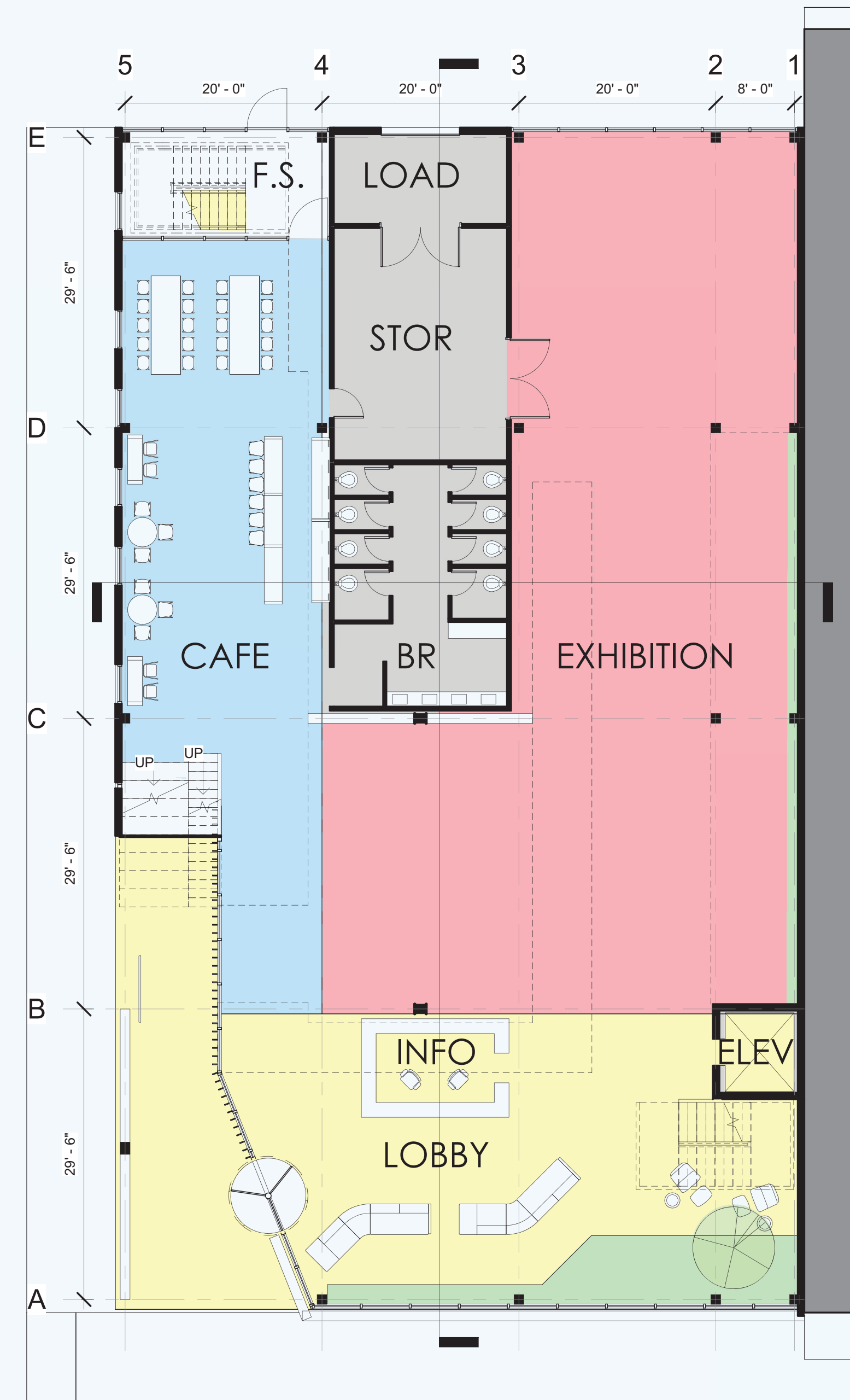
LEVEL 1 : 1/8" = 1'-0"
